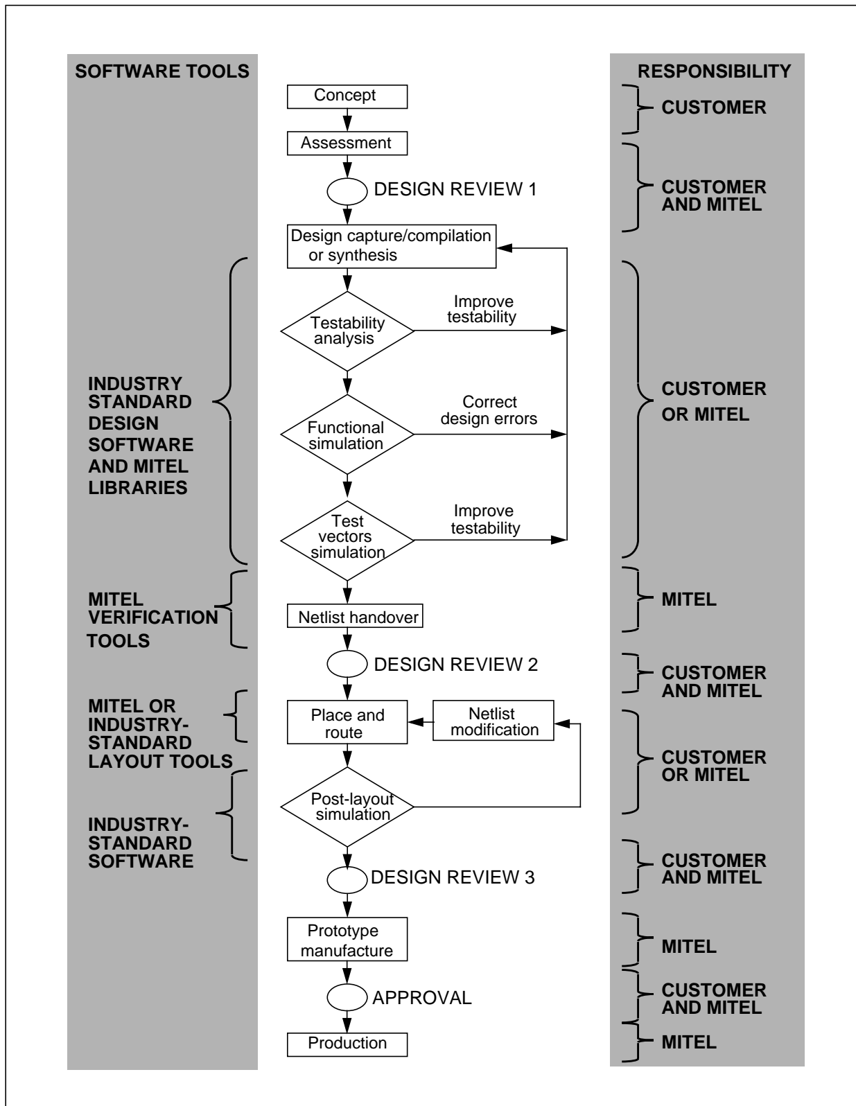
Figure 5 Design Flow
